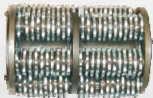
Hartmetallamellentrommel carbide tipped cutter drum
